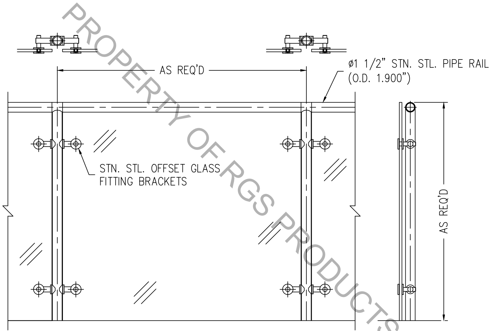
TYPICAL RAILING ELEVATION
